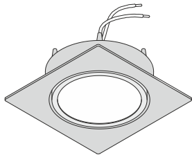
MODUS LED Art. 6421 24V 4W
