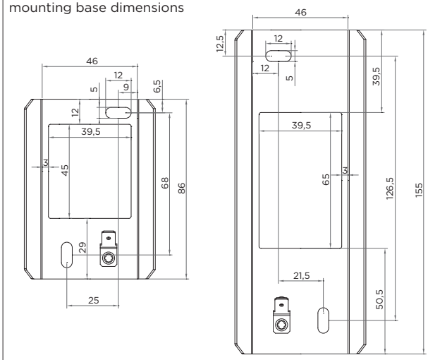
mounting base dimensions
