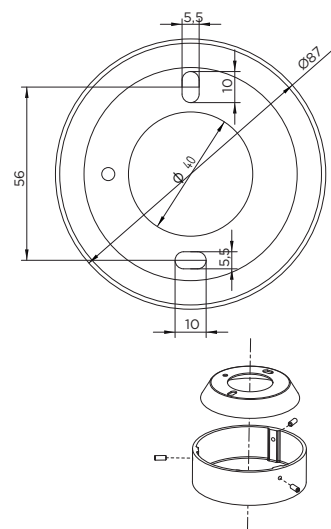
ceiling plate dimensions
