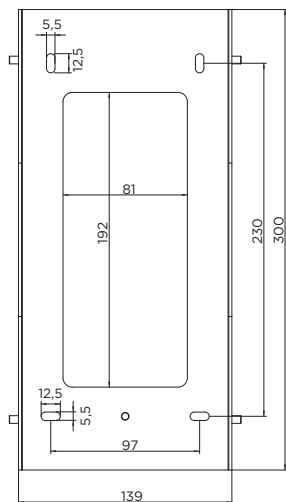
back plate dimensions
