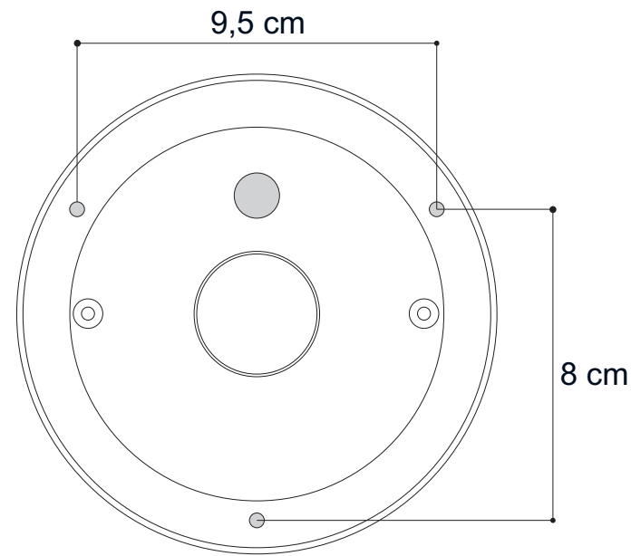
Interasse fori fissaggio Distance between fixing holes
