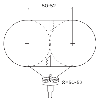
hole dimension
